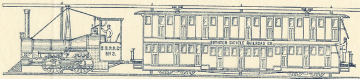
Engine No. 3. 2 Cylinders 12x14. Weight 16 Tons. 400 Tons Traction. 550 Revolutions per Minute. 5½ ft. Drivers. Speed: 100 Miles per hour.
